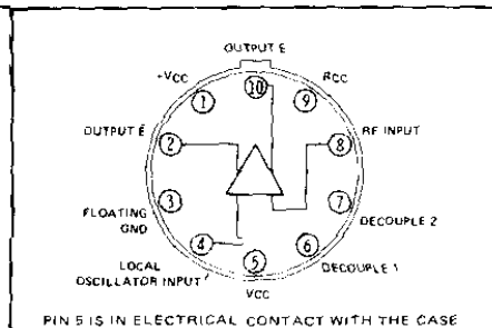
L PLUG-IN PACKAGE (TOP VIEW)
