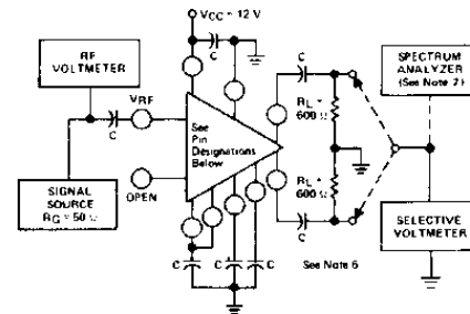
FIGURE 4— RFIF1
