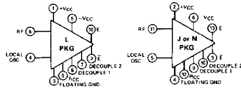
FIGURE 4— RFIF1
